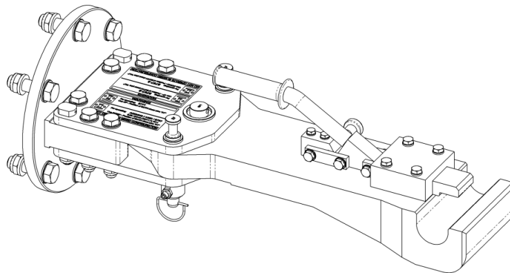
Shear pins in DOWN position
